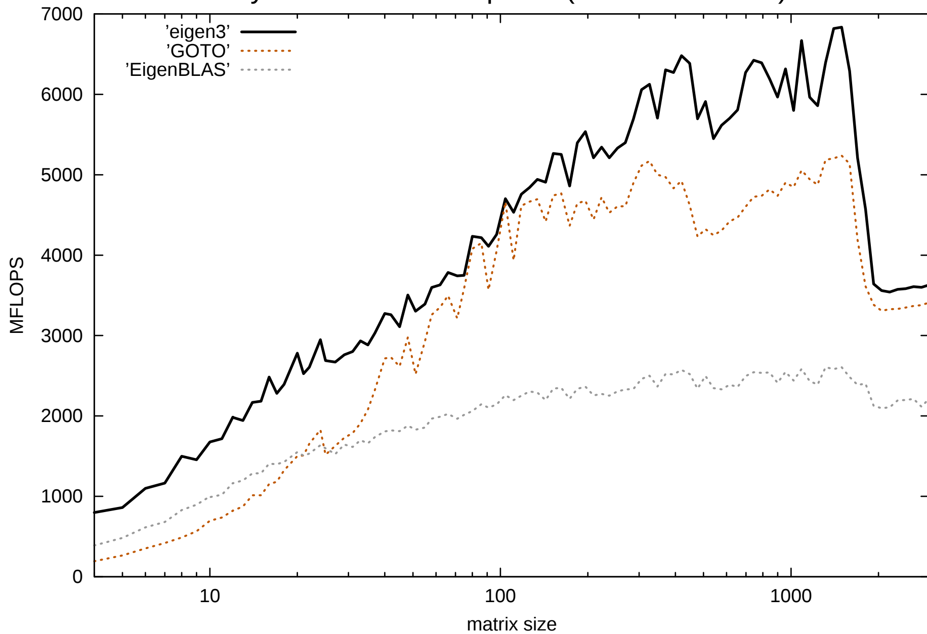
symmetric rank-2 update ( A += u^T v + u v^T )
