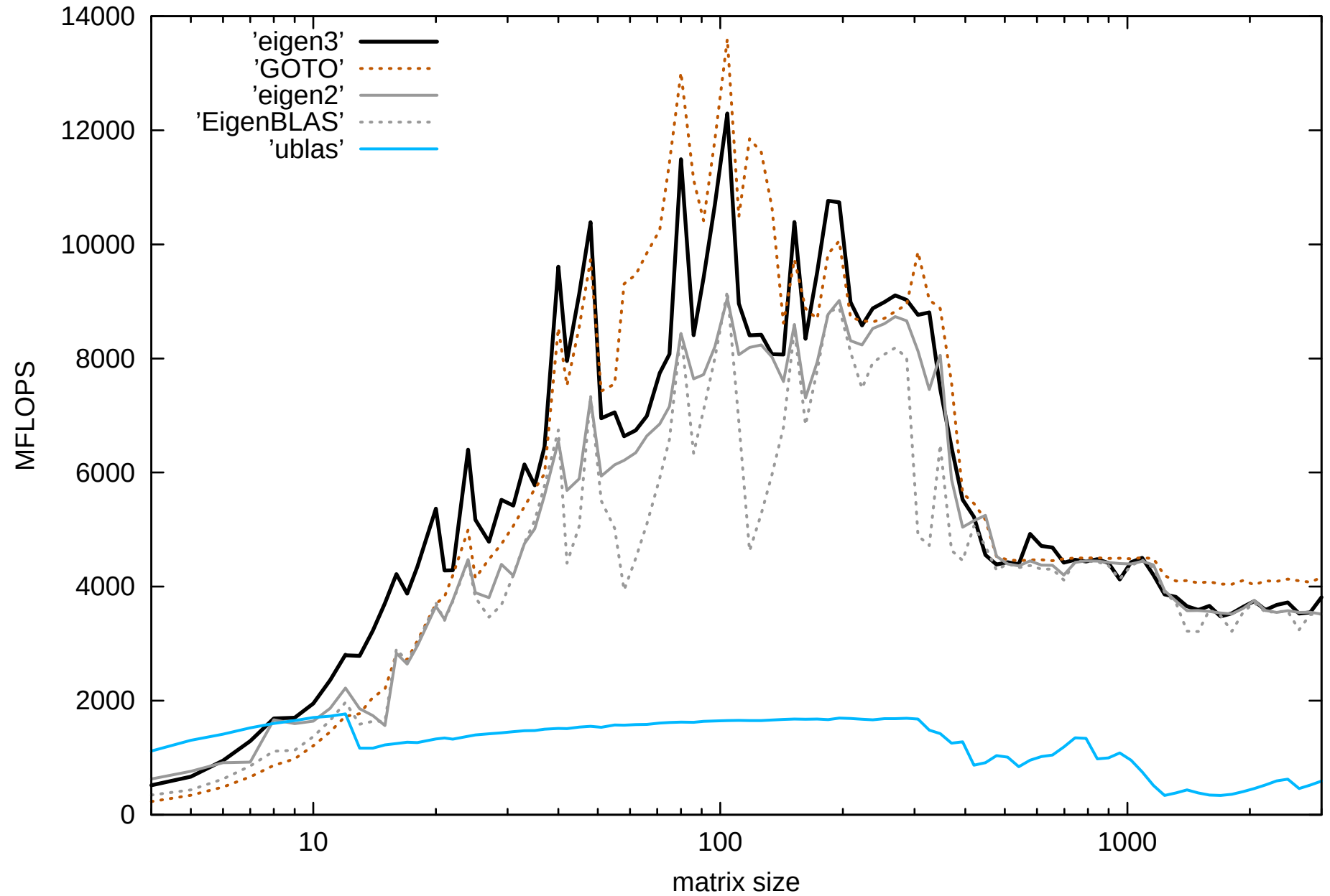
matrix vector product
