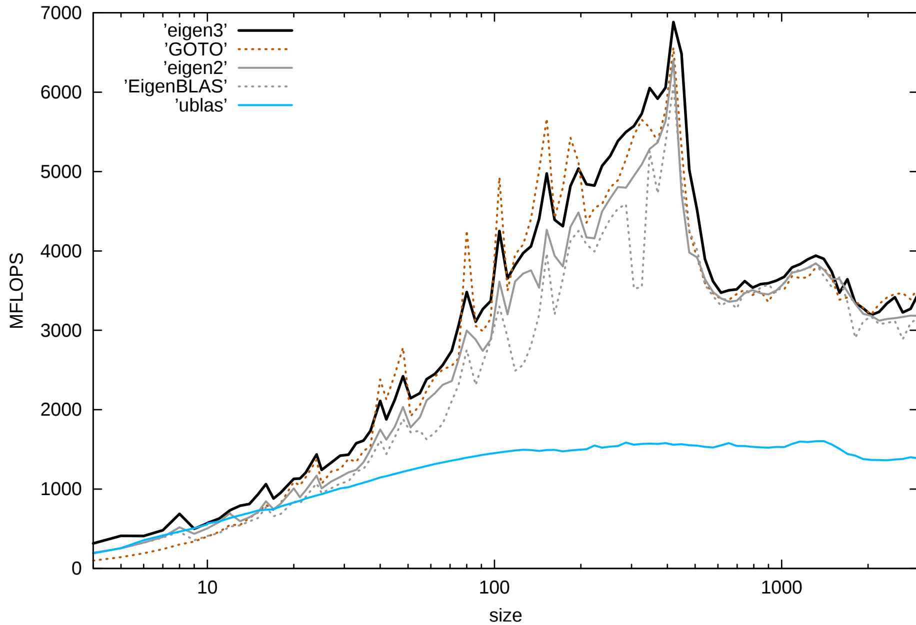
triangular solver - vector ( X = \text{inv}(L) X )
