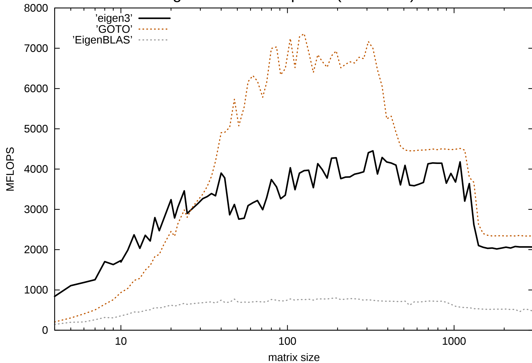
general rank-1 update ( A += u v^T )
